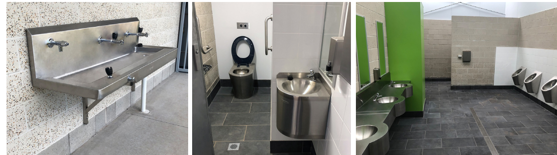
(L-R) Top: Britex Auto Mist Regal Urinals, Britex Accessible Hand Basin complete with Timed Flow Lever Tap and 300mm Side Shelf to fulfil AS1428 guidelines, Britex Wall Mounted Drinking Trough with Accessible end and compatible tapware, Britex Ambulant Cubicle featuring SS Ambulant Toilet Pan and Seat, Ambulant Grab Rails, In Wall Cistern and Actuator and Vandal Resistant Corner Hand Basin complete with Timed Flow Push Button Tapware, Britex bank of Curveline multibasins complete with Timed Flow Push Button tapware, also shown Auto Mist Regal Urinals.
