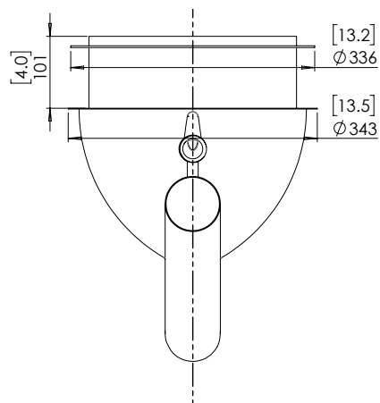
MODEL US-DW Front Elevation
