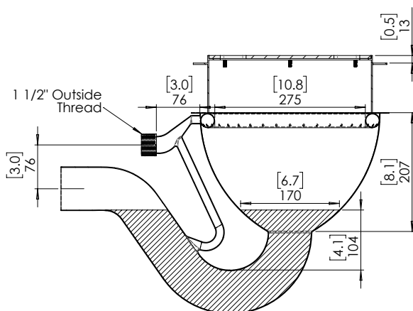
MODEL US-DW Side Elevation
