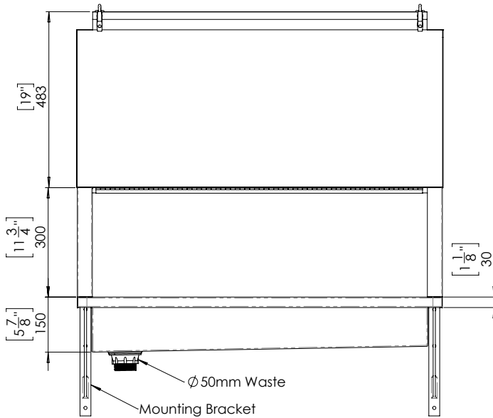
MODEL US-TLW Front Elevation
