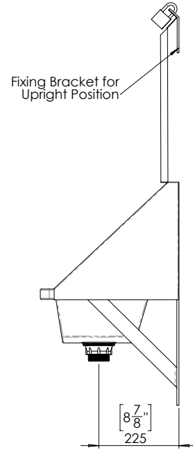
MODEL US-TLW Side Elevation
