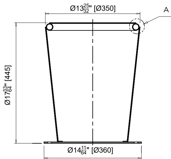
MODEL US-STL-SEC Front Elevation
