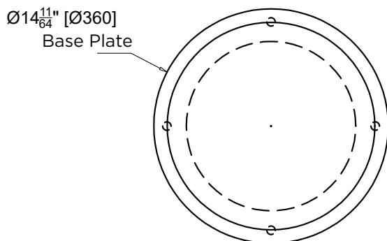
MODEL US-STL-SEC Plan
