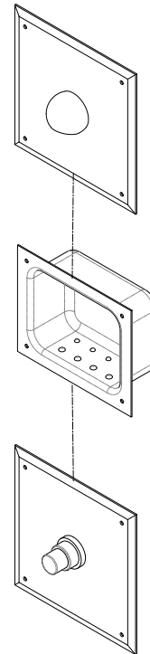
MODEL US-DWHC Isometric Views
