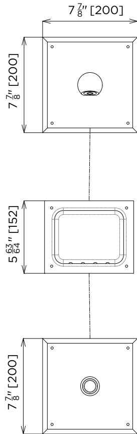
MODEL US-BSPF Front Elevations
