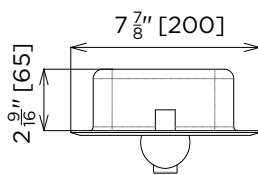
MODEL US-BSPF Plan
