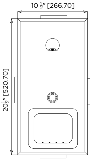
MODEL US-BSPR Front Elevation
