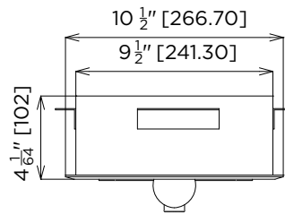
MODEL US-BSPR Plan
