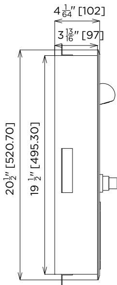
MODEL US-BSPR Side Elevation
