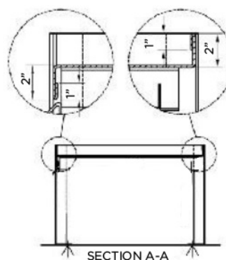
MODEL US-BUFS Side Elevation
