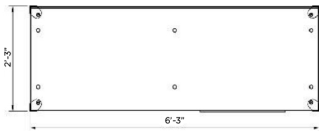
MODEL US-BUFS Plan Elevation
