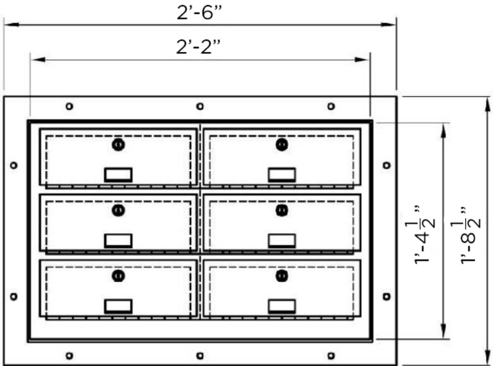
MODEL US-PLT Front Elevation
