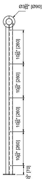
MODEL US-PPP Side Elevation
