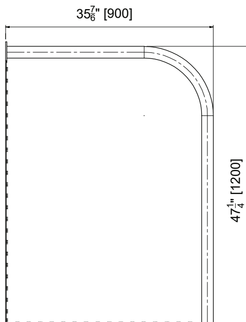
MODEL US-PPP Front Elevation
