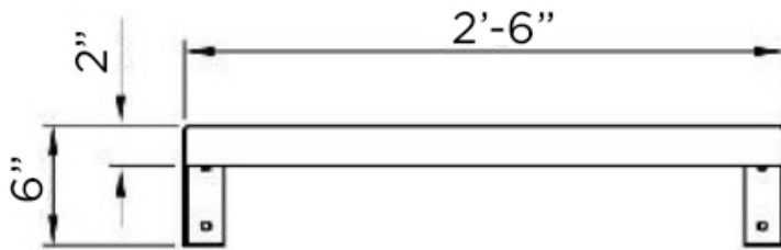
MODEL US-SDW Front Elevation
