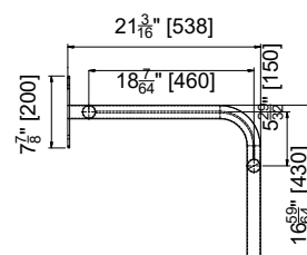
MODEL US-SWM-B Side Elevation
