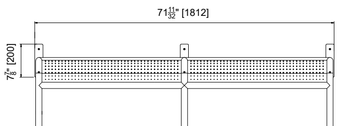
MODEL US-SWM-B Front Elevation
