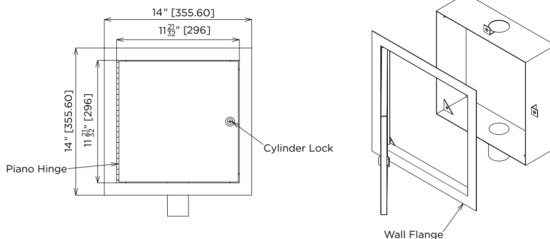
MODEL US-VBF Front Elevation & Isometric View
