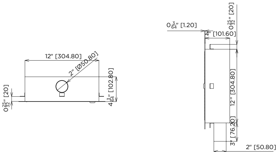
MODEL US-VBF Plan & Section
