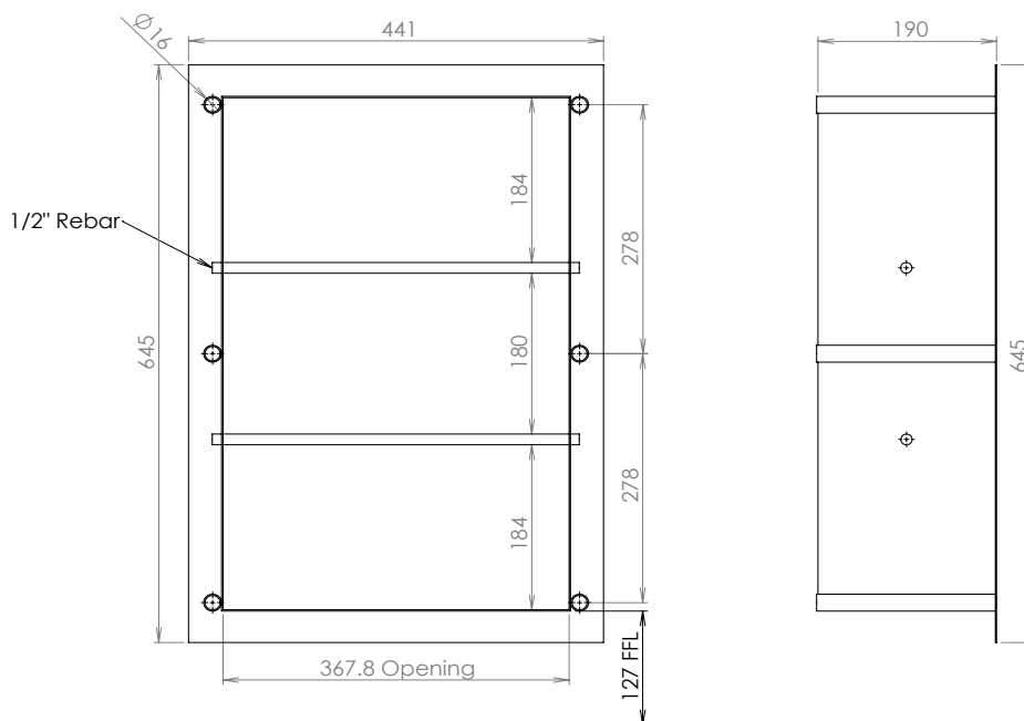
MODEL US-WS Front and Side Elevation
