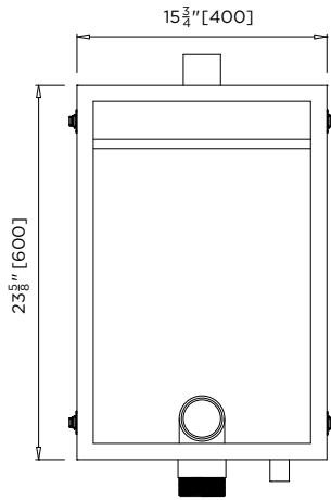
MODEL US-OSGI Plan
