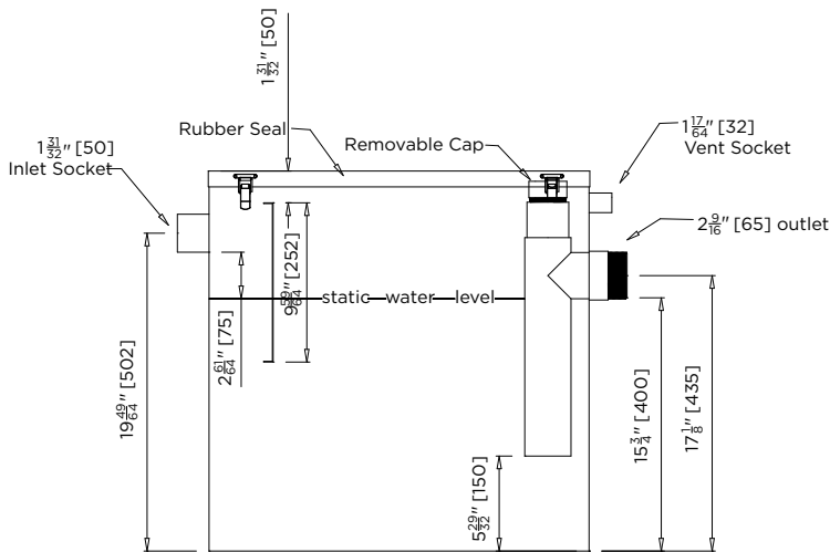
MODEL US-OSGI Side Elevation
