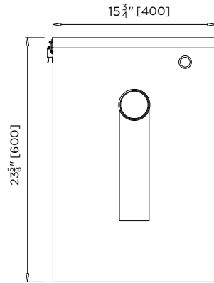
MODEL US-OSGI Front Elevation
