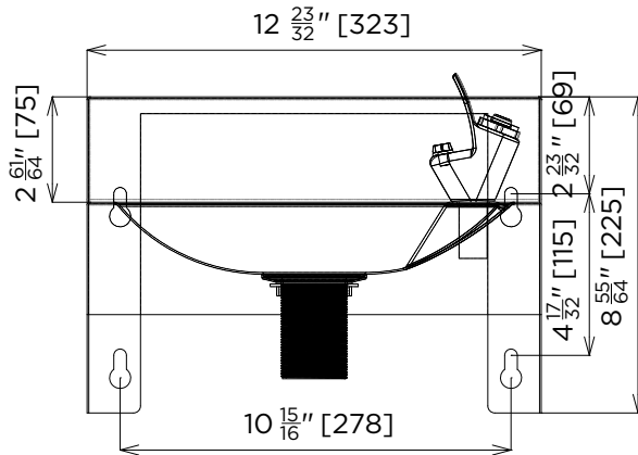
MODEL US-DWHC Front Elevation
