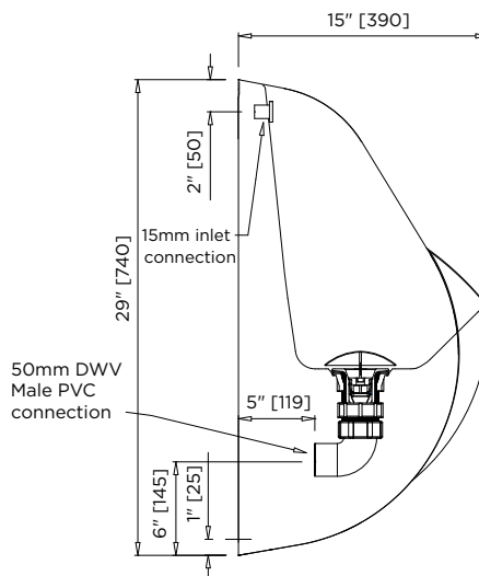
MODEL US-UAP Section
