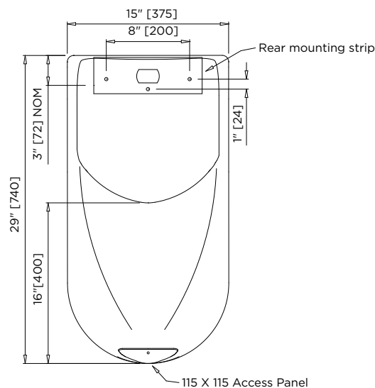
MODEL US-UAP Front Elevation
