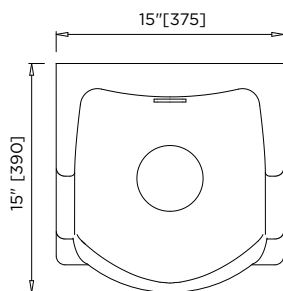
MODEL US-UAP Plan
