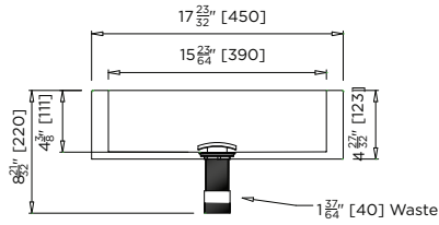
MODEL US-HBBEL-A Front Elevation
