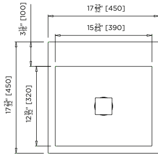
MODEL US-HBBEL-A Plan
