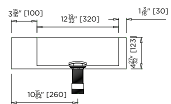
MODEL US-HBBEL-C Side Elevation
