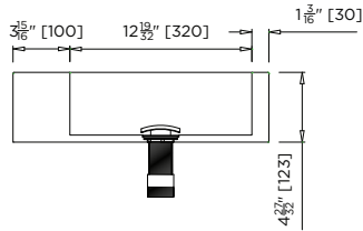
MODEL US-HBBEL-A Side Elevation
