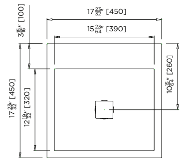
MODEL US-HBBEL-C Plan
