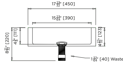
MODEL US-HBBEL-B Front Elevation
