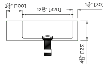
MODEL US-HBBEL-B Side Elevation
