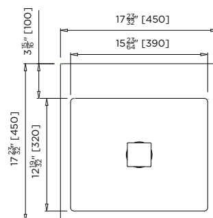
MODEL US-HBBEL-B Plan
