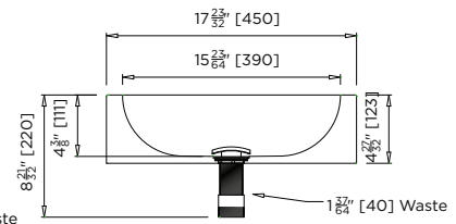
MODEL US-HBBEL-C Front Elevation
