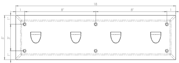
MODEL US-BTX-SH-004 Front Elevation
