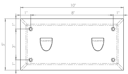
MODEL US-BTX-SH-002 Front Elevation
