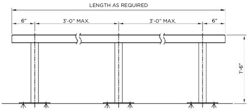
MODEL US-FMBC Front Elevation
