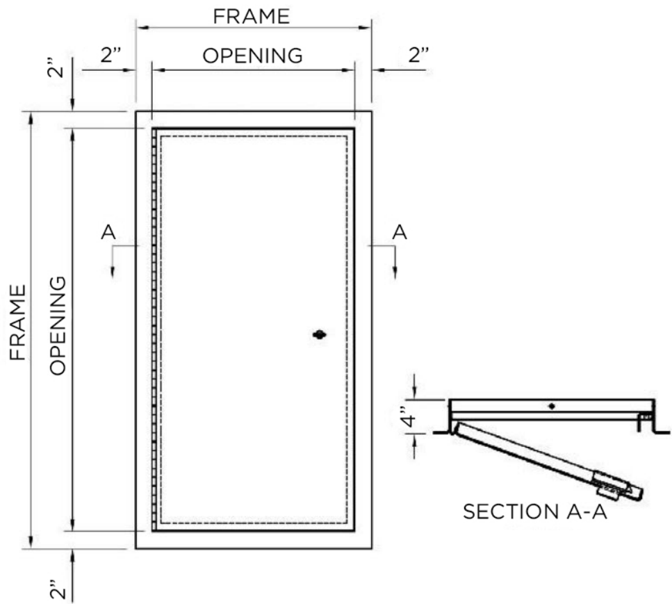
MODEL US-SAP Front Elevation
