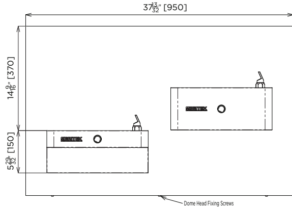
MODEL US-DDS2 Front Elevation
