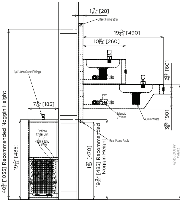
MODEL US-DDS2 Side Elevation
