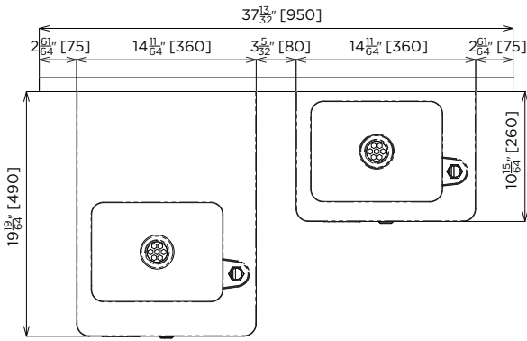
MODEL US-DDS2 Plan
