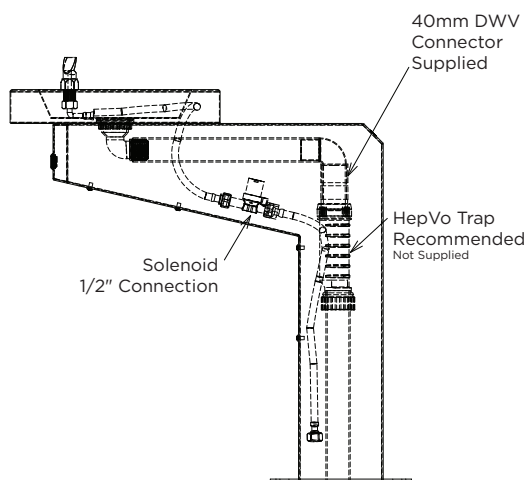
MODEL US-DDIS Side Elevation
