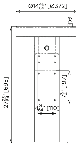
MODEL US-DDIS Front Elevation
