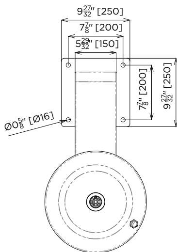
MODEL US-DDIS Plan
