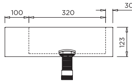
MODEL HBBEL-A Side Elevation
