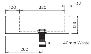
MODEL HBBEL-C Side Elevation
