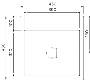
MODEL HBBEL-A Plan
