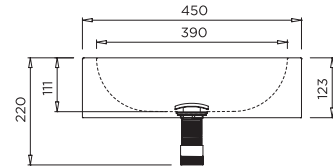
MODEL HBBEL-C Front Elevation
