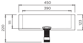
MODEL HBBEL-A Front Elevation
