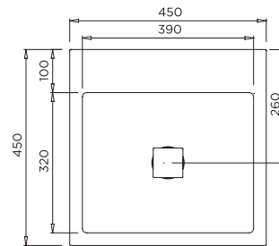
MODEL HBBEL-B Plan
