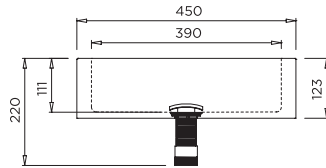
MODEL HBBEL-B Front Elevation
