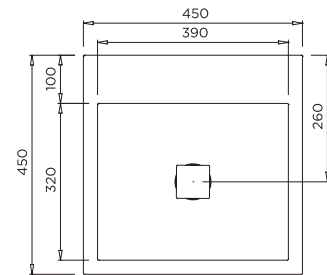
MODEL HBBEL-C Plan
