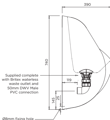
MODEL UAPM Section and Front Elevation
