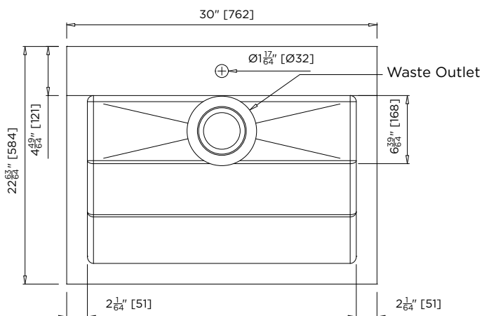
MODEL US-ST1 Plan
