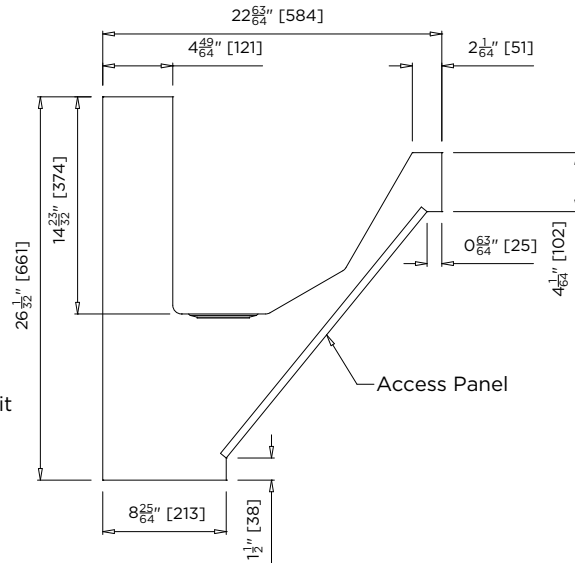
MODEL US-ST1 Section
