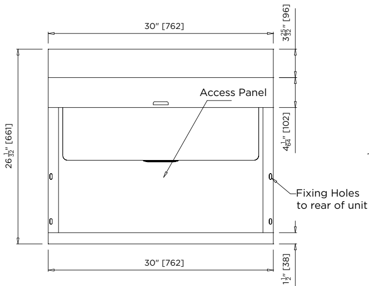
MODEL US-ST1 Front Elevation
