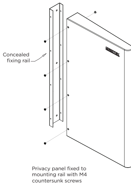
MODEL US-UPP Isometric View
