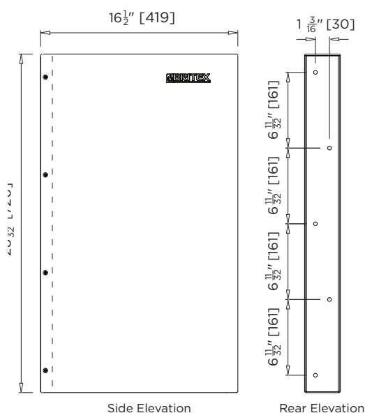
MODEL US-UPP Side and Rear Elevation
