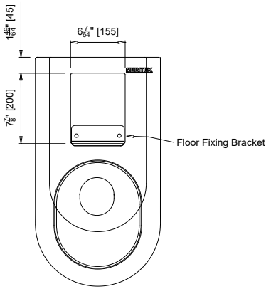
MODEL US-PCAMS / P Plan
