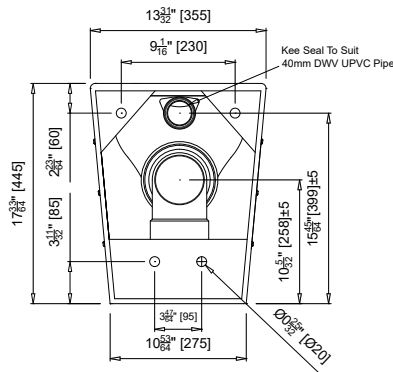
MODEL US-PCAMS Side and Rear Elevation
