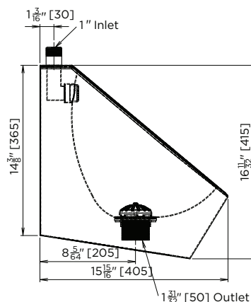
MODEL US-UWHU Section
