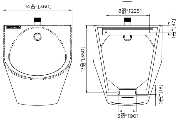
MODEL US-UWHU Front and Rear Elevation
